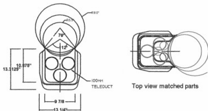
95-3-Way PILASTER Plan View
