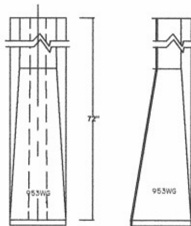
95-3-Way GUARD Elevation
