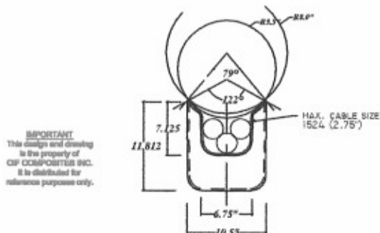
95-3-Way GUARD Top View
