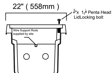
END ELEVATION section at centre
