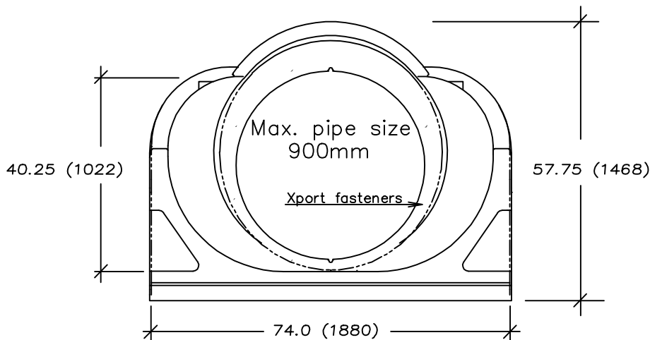
4 Series Xport Headwall Low Profile
